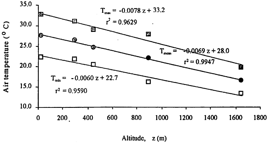
Figure 1. Relationships between altitude and minimum ( T_{\min} ), averaged ( T_{\text{mean}} ) and maximum ( T_{\max} ) air temperatures.
